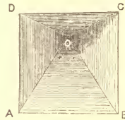
Fig. 5.—Tetrahedral Angle.
